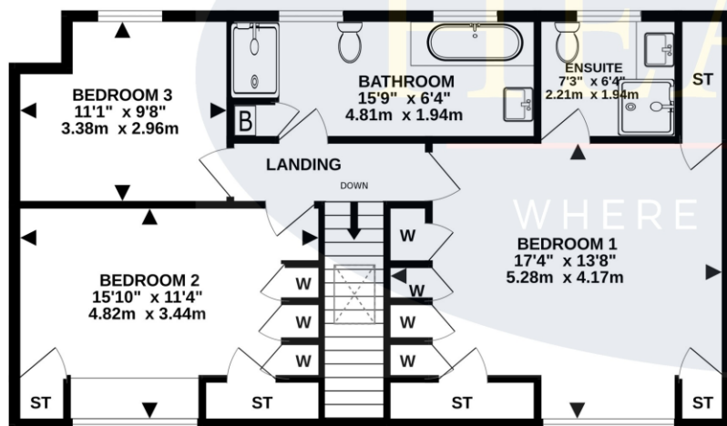
1ST FLOOR 762 sq.ft. (70.8 sq.m.) approx.
