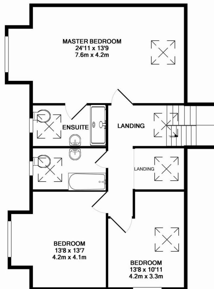
1ST FLOOR APPROX. FLOOR AREA 927 SQ.FT. (86.1 SQ.M.)
